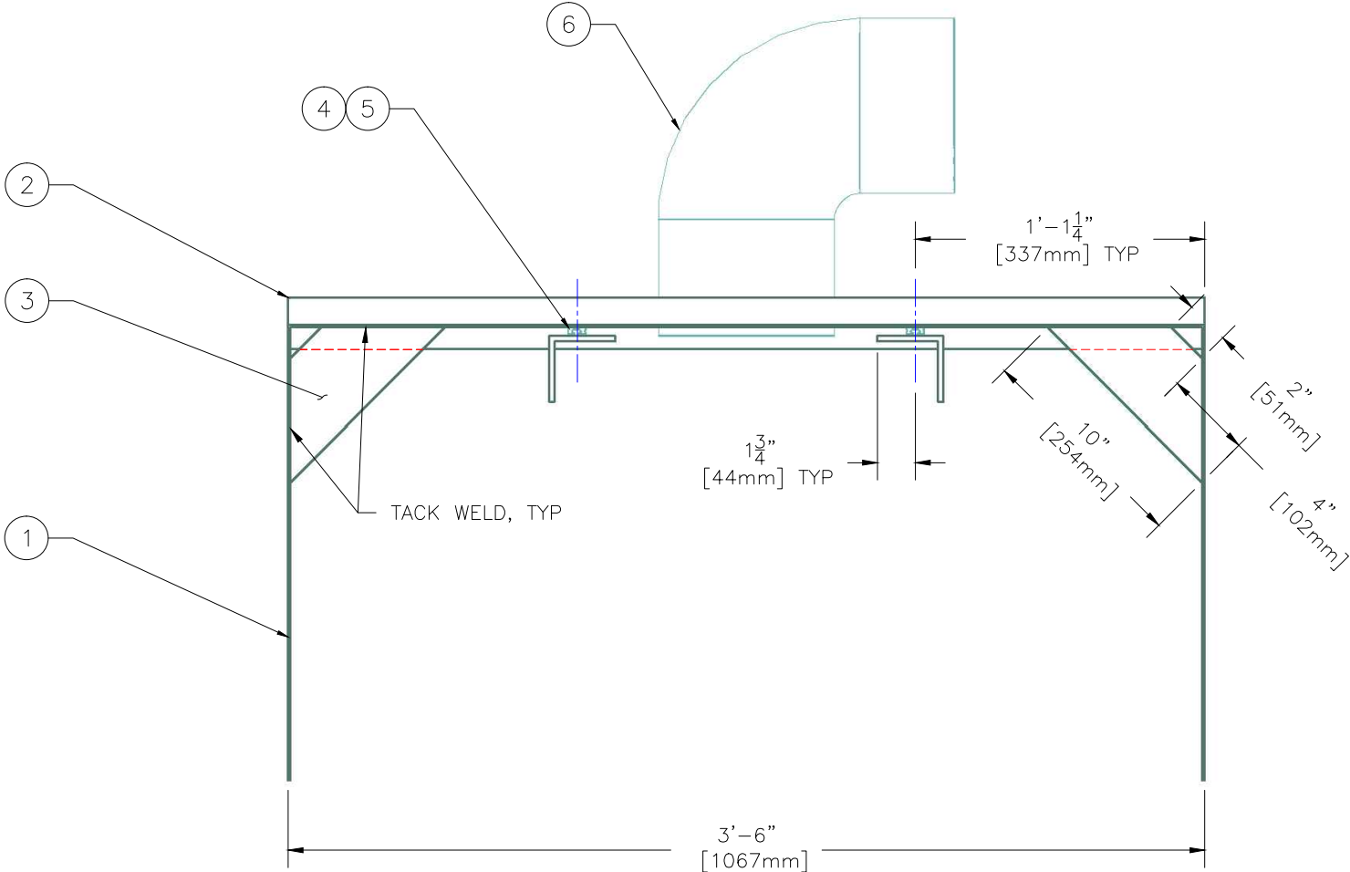
FIELD DRILL BOLT HOLES ON ANGLES AND PN 1
