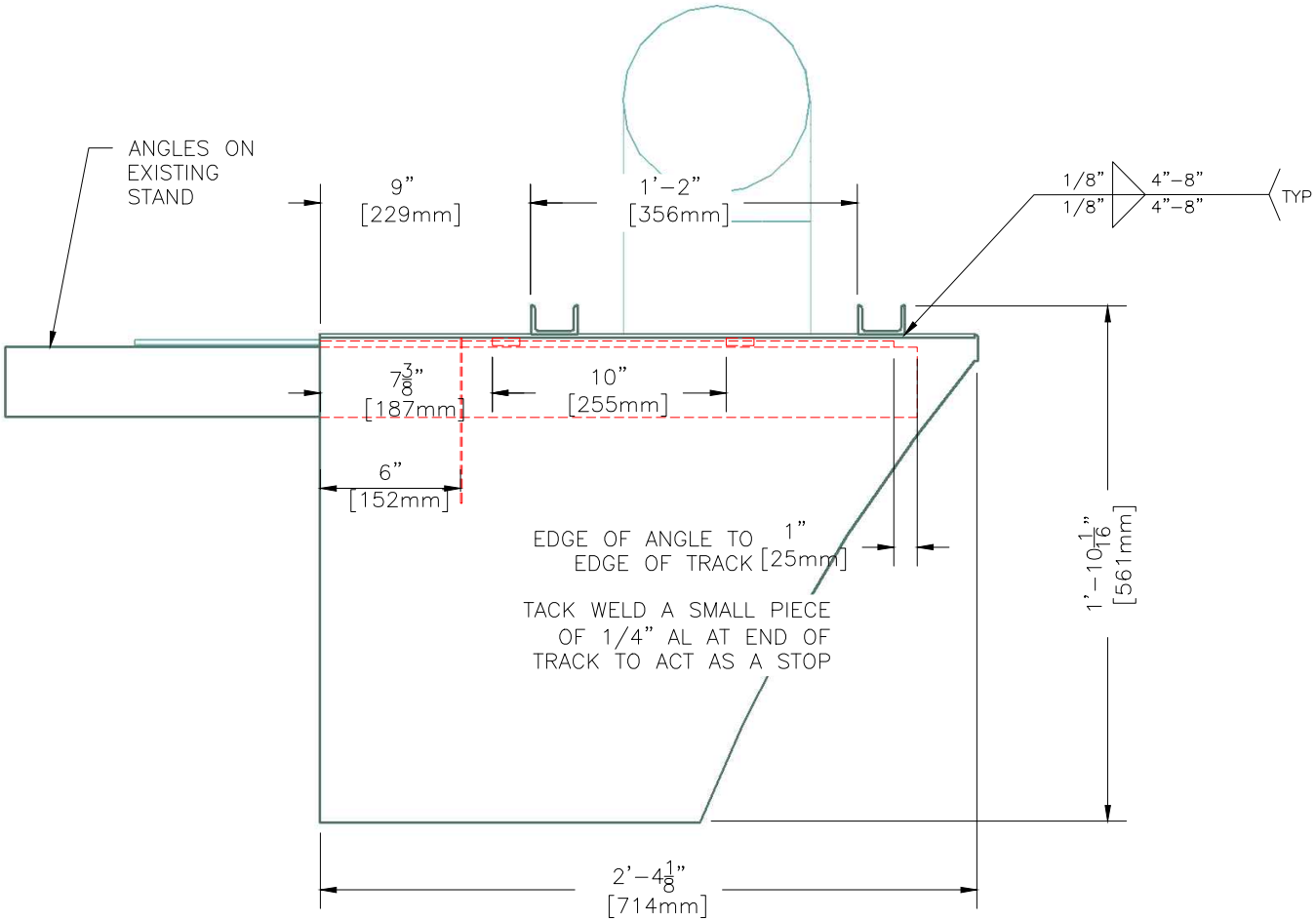
FIELD DRILL BOLT HOLES ON ANGLES AND PN 1
